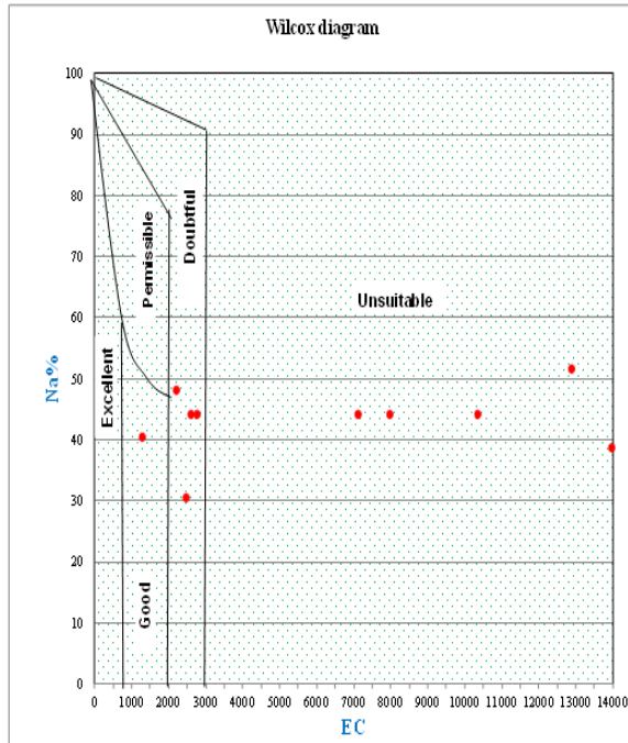
Figure (2): Wilcox diagram relating Na% and EC. Doneen Diagram
